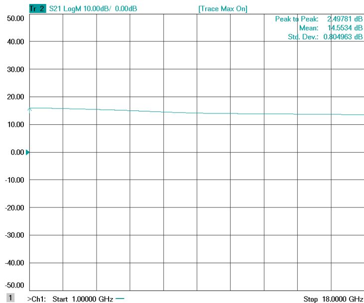
Figure 2: ERZ-HPA-0100-1800-21 Small Signal Gain
