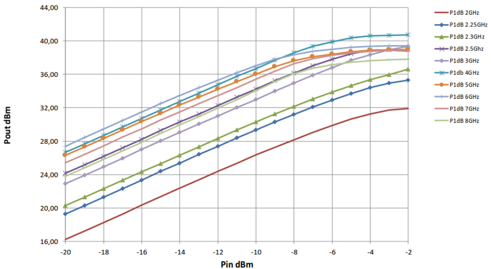
Figure 2: ERZ-HPA-0200-0800-36 P1dB Vs Pin
