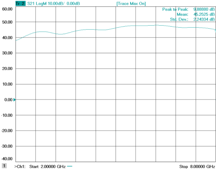
Figure 3: ERZ-HPA-0200-0800-36 Small Signal Gain
