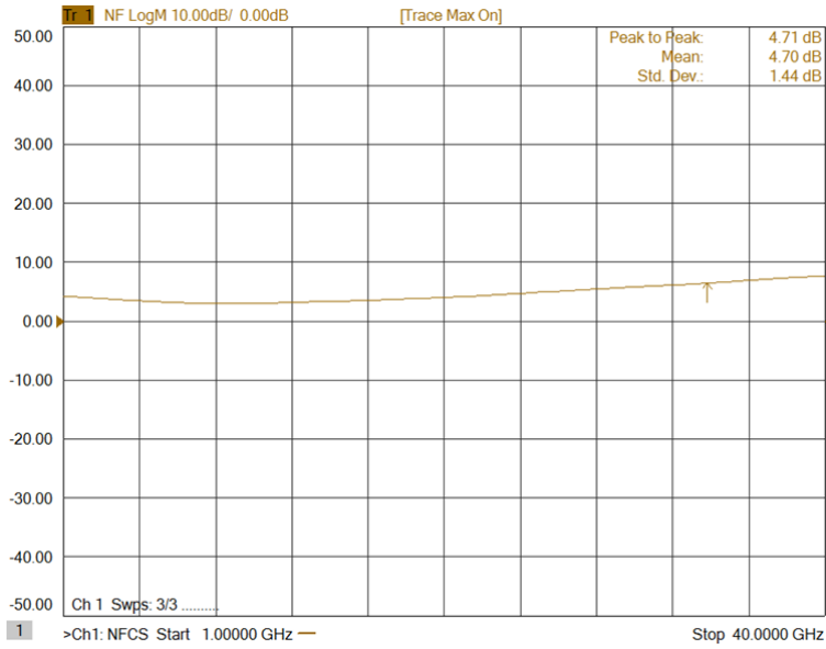
Figure 3: ERZ-LNA-1800-4000-15-4 Noise Figure
