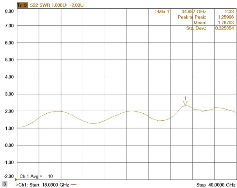
Figure 5: ERZ-LNA-1800-4000-15-4 Output Matching
