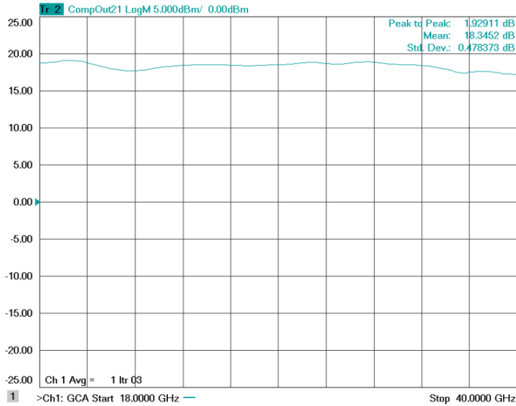
Figure 1: ERZ-LNA-1800-4000-15-4 P1dB
