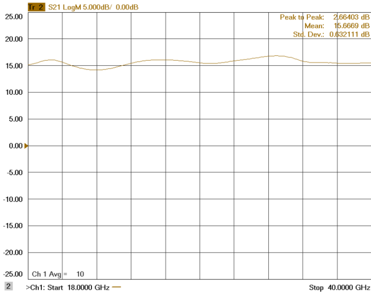
Figure 2: ERZ-LNA-1800-4000-15-4 Small Signal Gain
