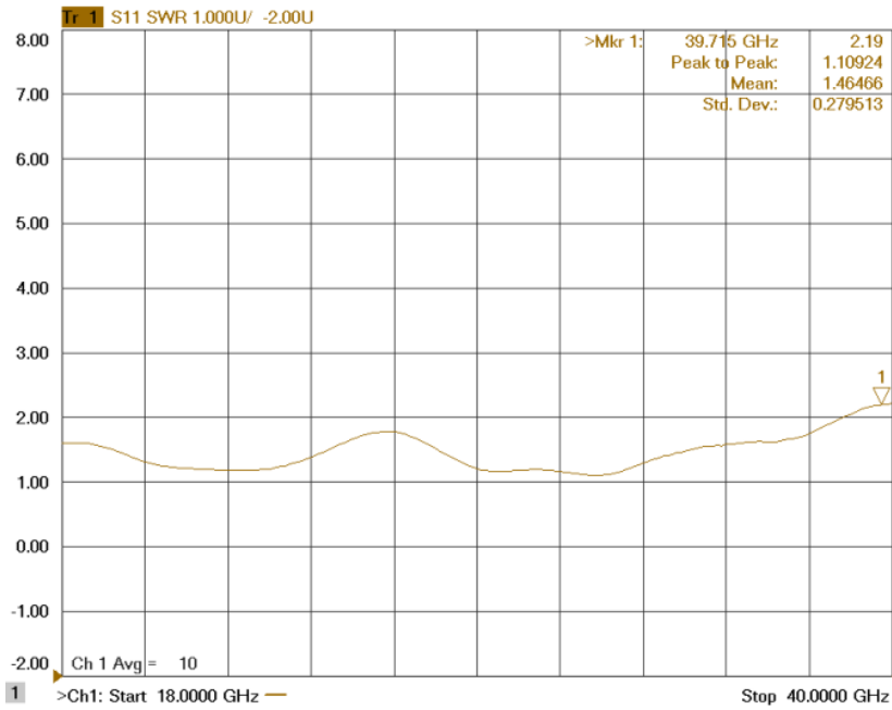
Figure 4: ERZ-LNA-1800-4000-15-4 Input Matching
