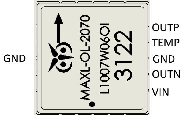
Figure 3 Pinout Description (Top View)
